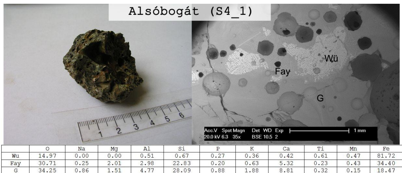
Fig. 10. Slag sample S4_1 from Alsóbogát bloomery workshop.
