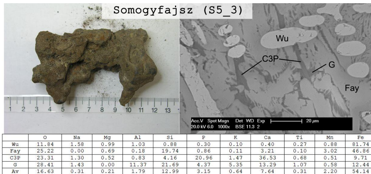
Fig. 14. Slag sample S5_3 from Somogyfajsz bloomery workshop.
