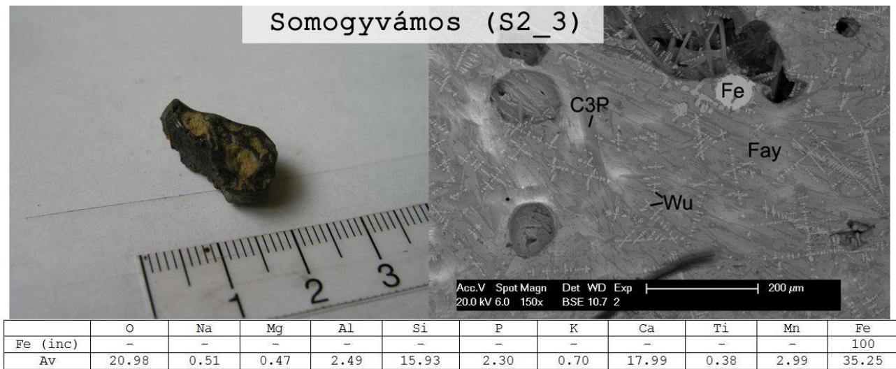
Fig. 8. Slag sample S2_3 from Somogyvámos bloomery workshop.
