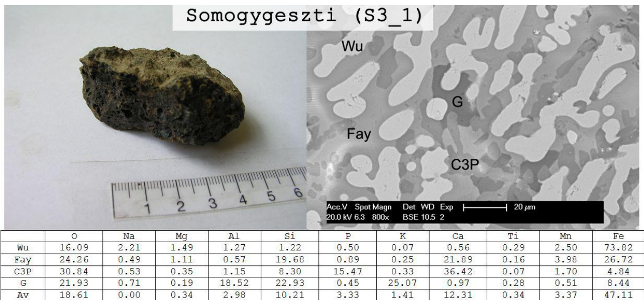
Fig. 9. Slag sample S3_1 from Somogygeszti bloomery workshop.
