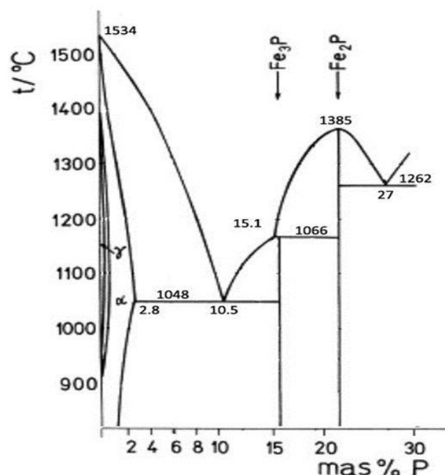
Fig. 1. Fe-P dual phase diagram
