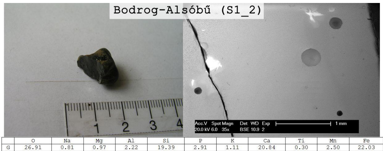
Fig. 4. Slag sample S1_2 from Bodrog-Alsóbü bloomery workshop.
