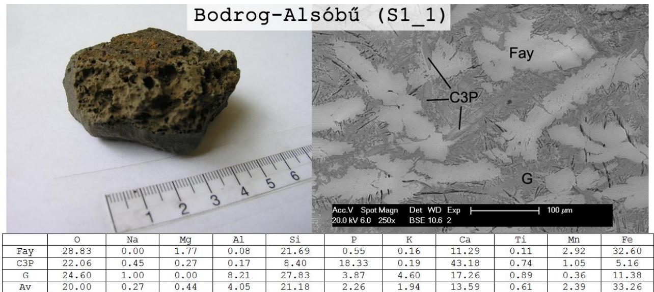
Fig. 3. Slag sample S1_1 from Bodrog-Alsóbü bloomery workshop. Left: The sample. Right: SEM picture of the sample and the observed microstructures. Bottom: Table of the EDS results. In the table elements in wt%, Wü – wustite, Fay – fayalite, C3P – tricalcium-phosphate, G – glass, Av – average, Fe(inc) – iron inclusion.
