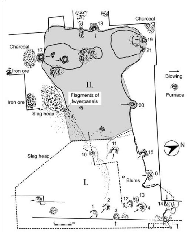
Fig. 3 - Somogyfajsz. Ground plan of the bloomery workshops Nr. I and Nr. II. End of the 10th century A.D. Workshop Nr. II is visible in situ in the „Őskohó Múzeum” (Bloomery Museum)
